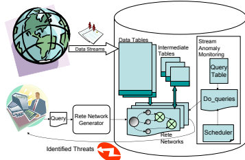
Fig. 1. ARGUS System Architecture
