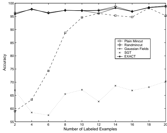
Figure 2. "1" vs "2" on the digits dataset with the MST graph (left) and \delta_{\frac{1}{4}} graph (right).
