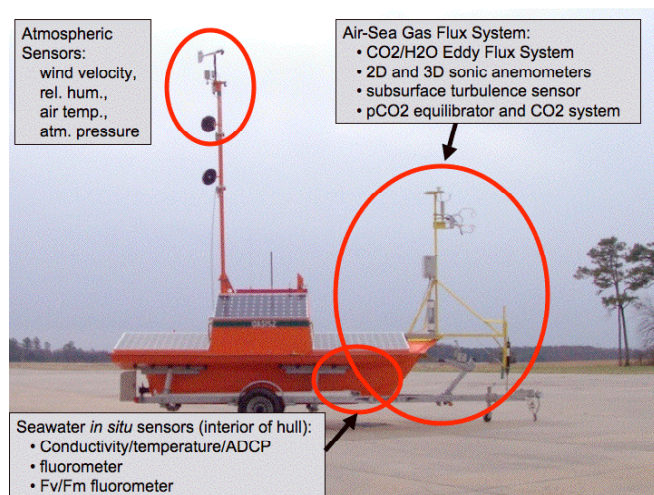
Fig. 4. The OASIS boat with its primary sensor systems.
