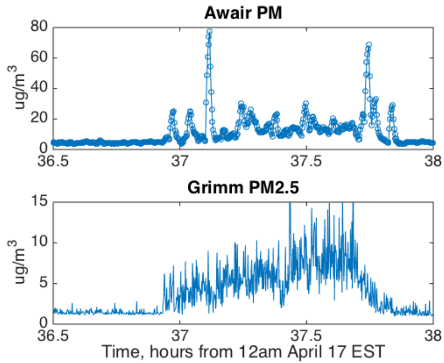
Figure 5.20: Awair vs. Grimm particle concentration, 1.5-hour interval
