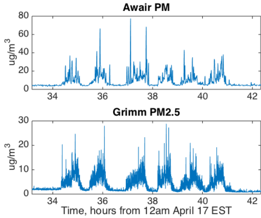
Figure 5.19: Awair vs. Grimm particle concentration, 9-hour interval
