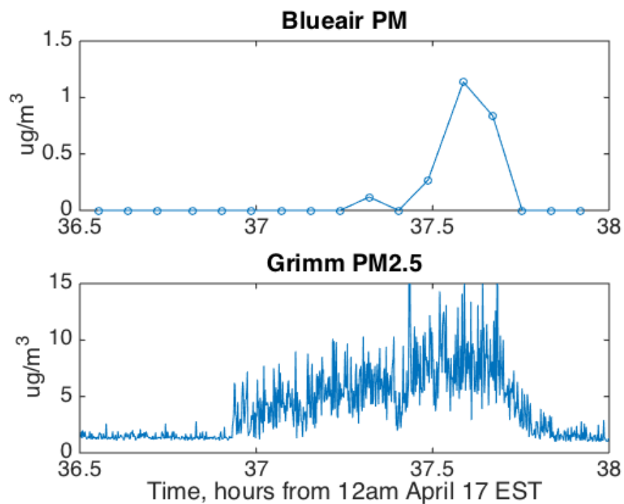
Figure 5.26: Blueair Aware vs. Grimm particle concentration, 1.5-hour interval
