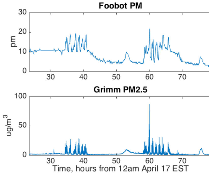
Figure 5.21: Foobot vs. Grimm particle concentration, 55-hour interval
