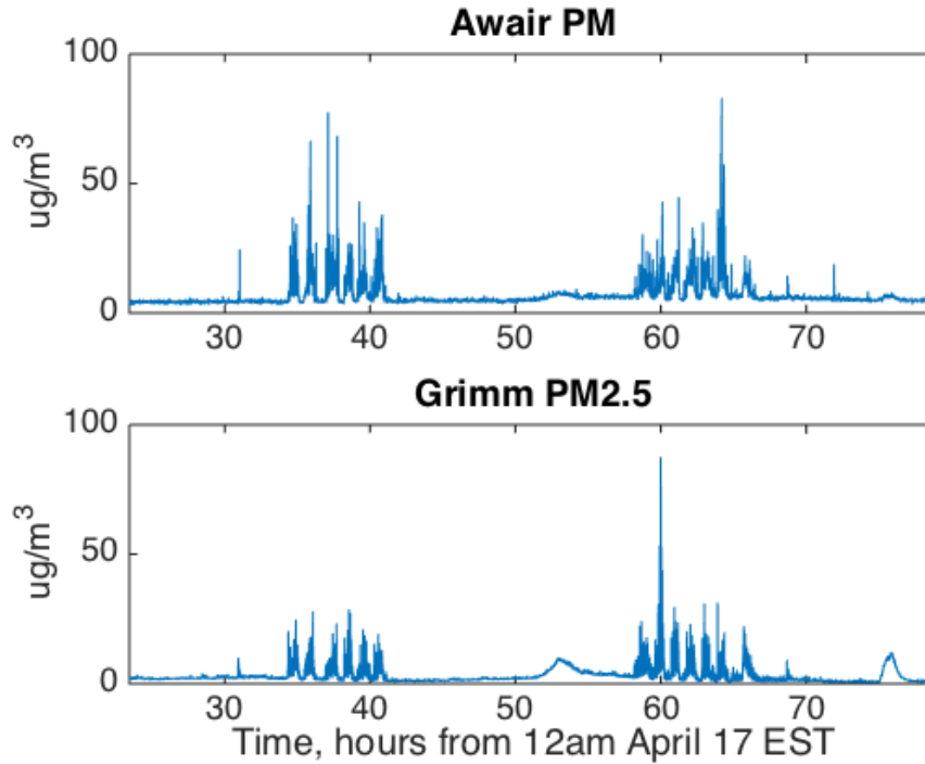
Figure 5.18: Awair vs. Grimm particle concentration, 55-hour interval
