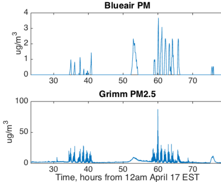
Figure 5.24: Blueair Aware vs. Grimm particle concentration, 55-hour interval
