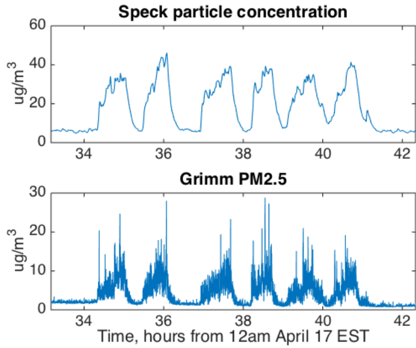
Figure 5.13: Speck vs. Grimm particle concentration, 9-hour interval
