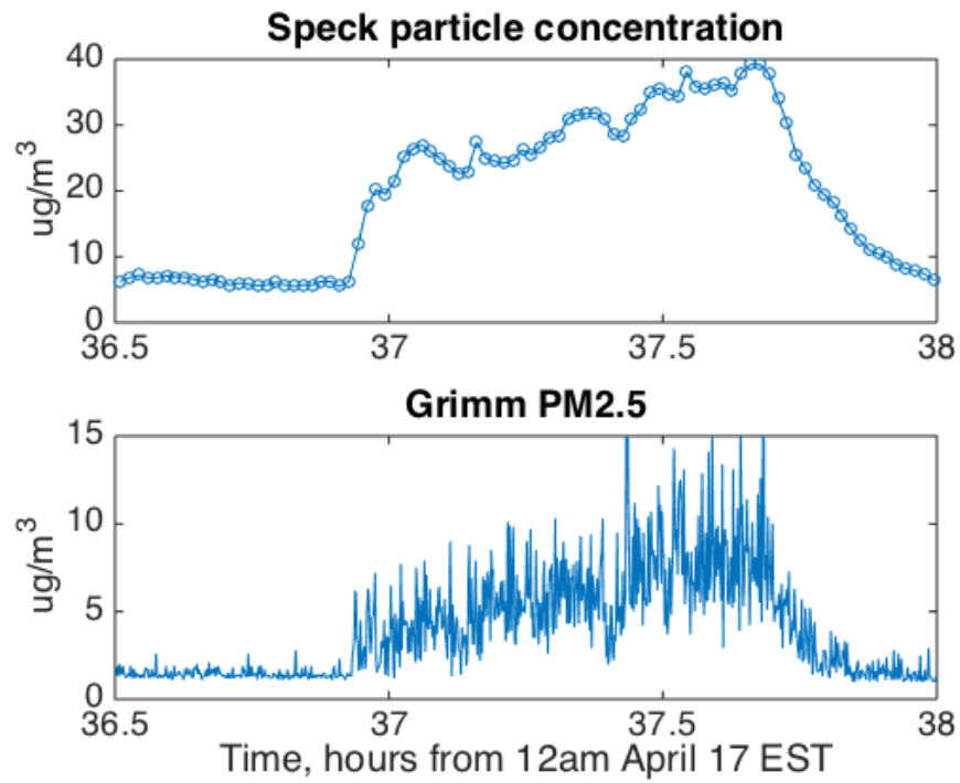
Figure 5.14: Speck vs. Grimm particle concentration, 1.5-hour interval
