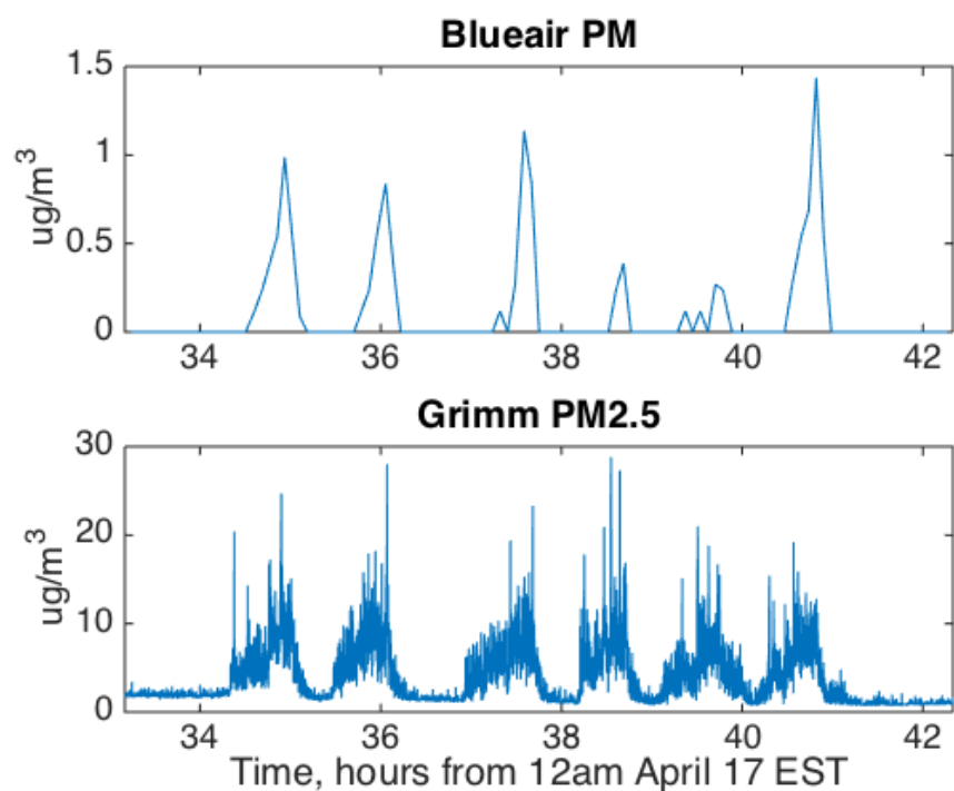
Figure 5.25: Blueair Aware vs. Grimm particle concentration, 9-hour interval
