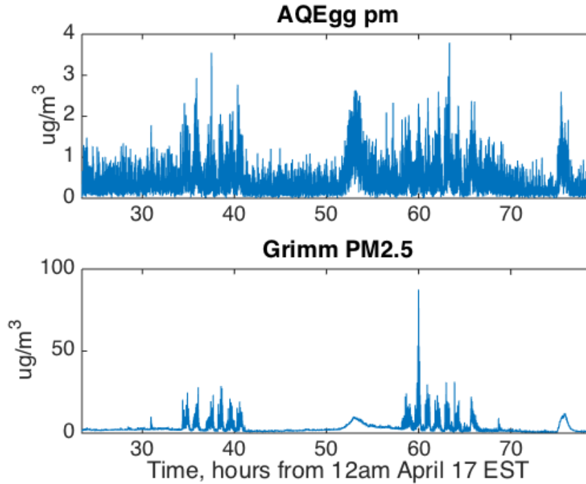
Figure 5.15: Air Quality Egg vs. Grimm particle concentration, 55-hour interval
