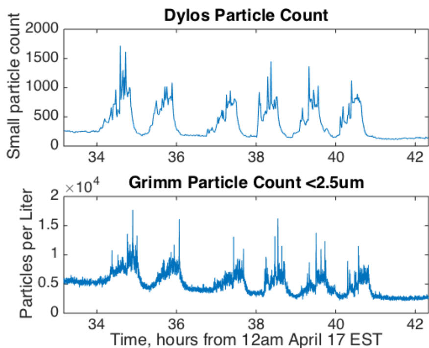
Figure 5.28: Dylos vs. Grimm particle count, 9-hour interval
