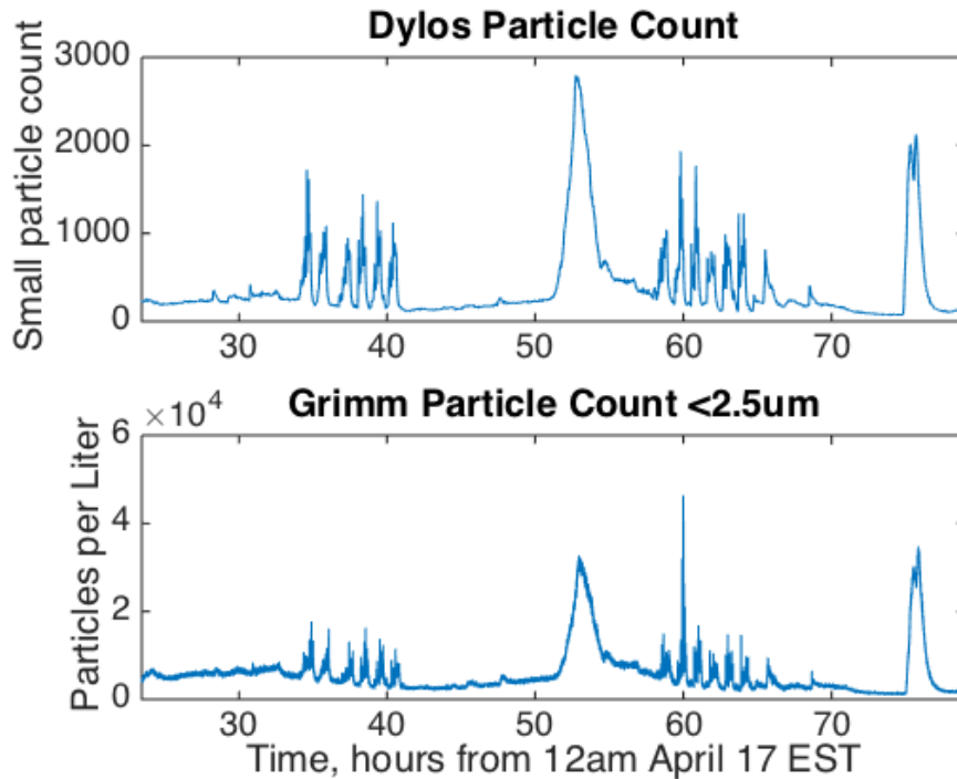
Figure 5.27: Dylos vs. Grimm particle count, 55-hour interval
