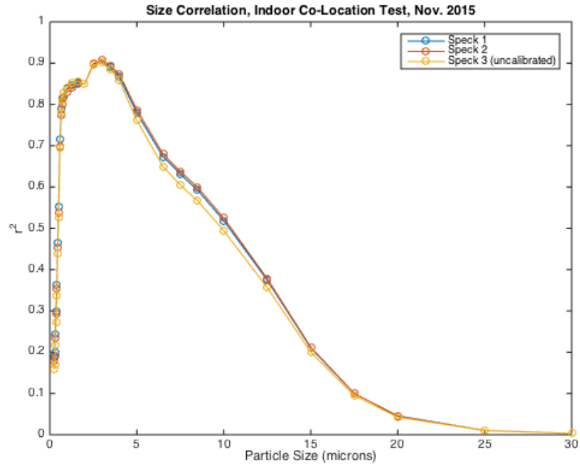
Figure 5.6: Plot of Speck correlation values with respect to particle diameter, demonstrating size sensitivity
