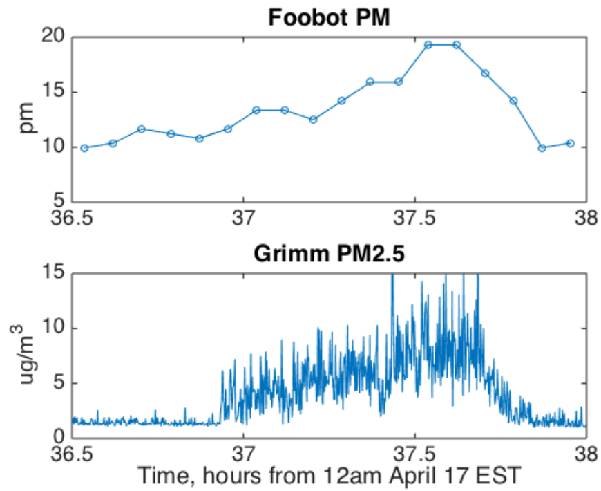
Figure 5.23: Foobot vs. Grimm particle concentration, 1.5-hour interval
