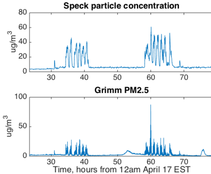
Figure 5.12: Speck vs. Grimm particle concentration, 55-hour interval
