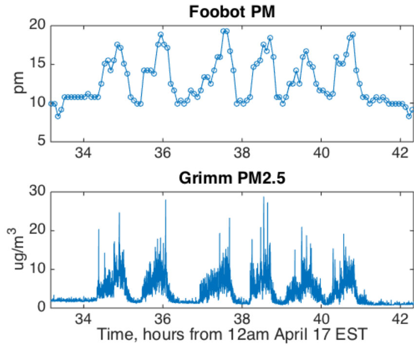
Figure 5.22: Foobot vs. Grimm particle concentration, 9-hour interval
