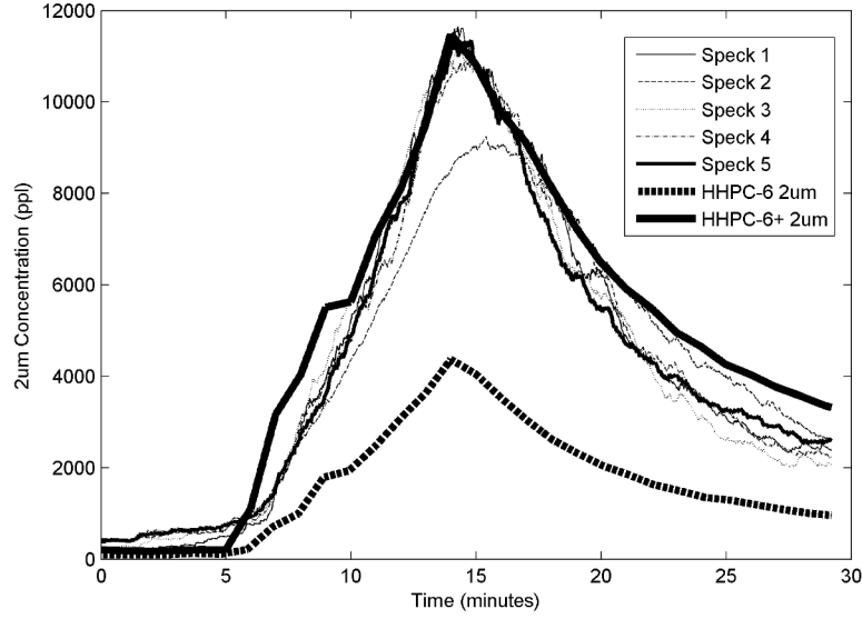
Figure 4.2: Plot of calibration data over time. Note the large discrepancy between the HHPC-6 channels.
