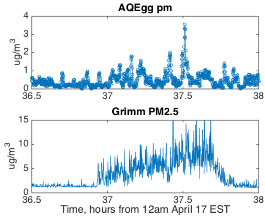
Figure 5.17: Air Quality Egg vs. Grimm particle concentration, 1.5-hour interval
