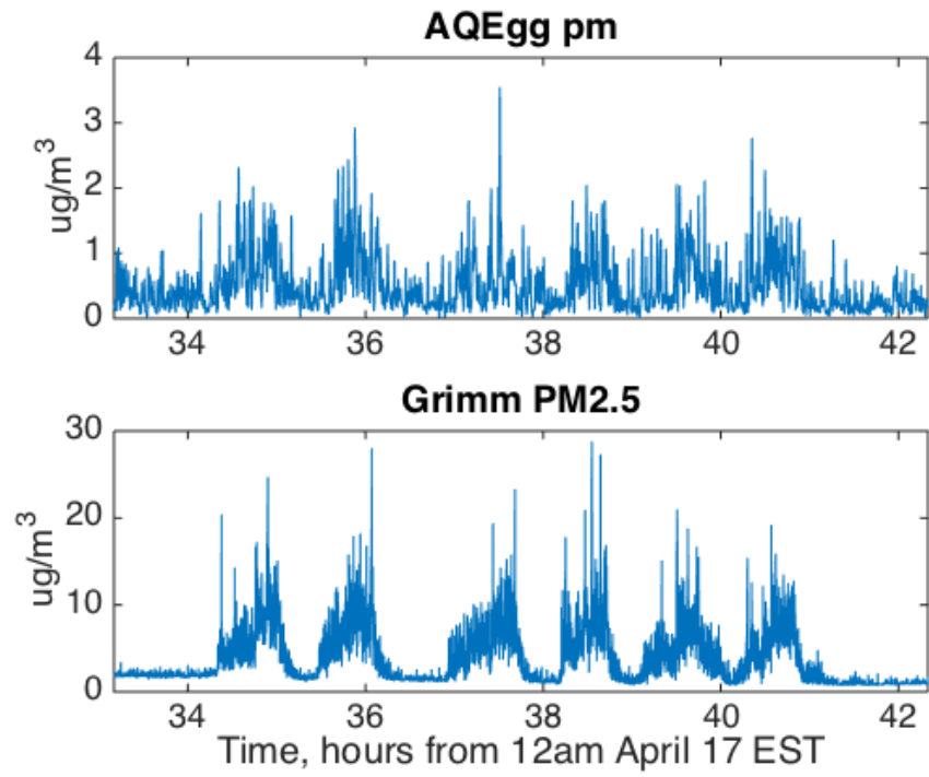
Figure 5.16: Air Quality Egg vs. Grimm particle concentration, 9-hour interval
