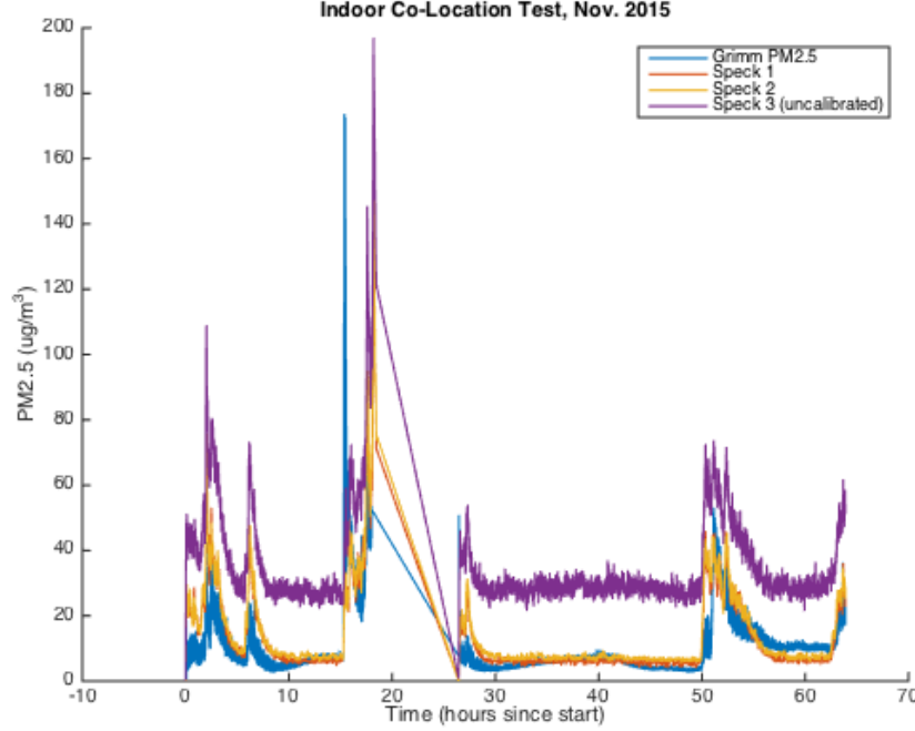
Figure 5.4: Plot of kitchen co-location experiment with three Specks and one grimm EDM180
