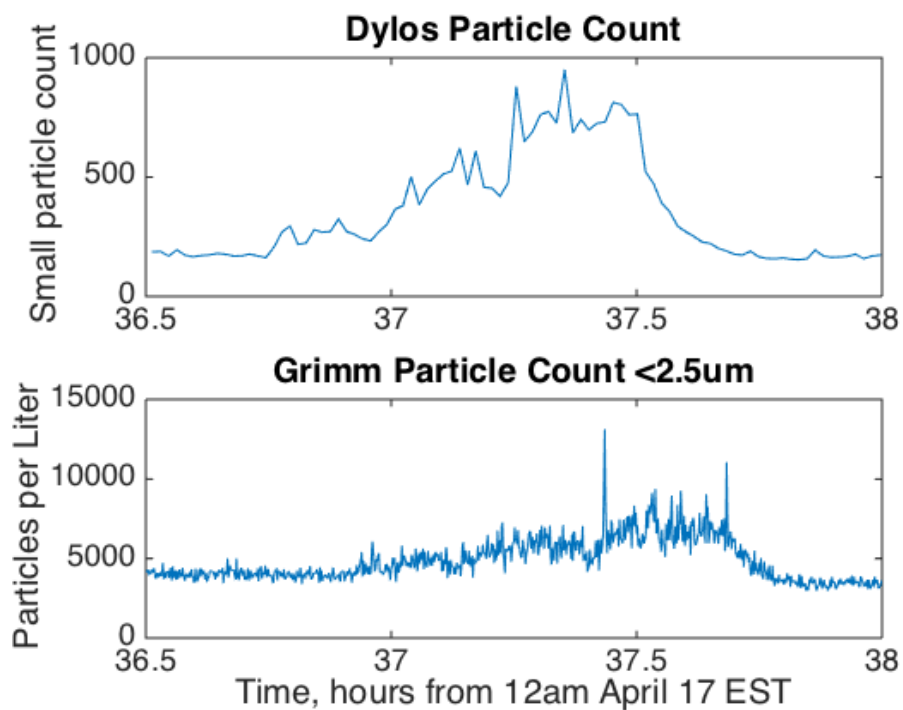
Figure 5.29: Dylos vs. Grimm particle count, 1.5-hour interval
