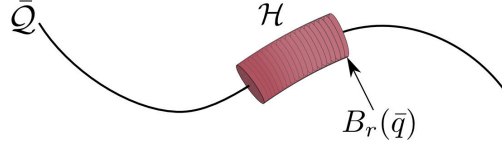
Figure 9.4: A self-motion manifold in C-space. r = 2 and n = 3 .
