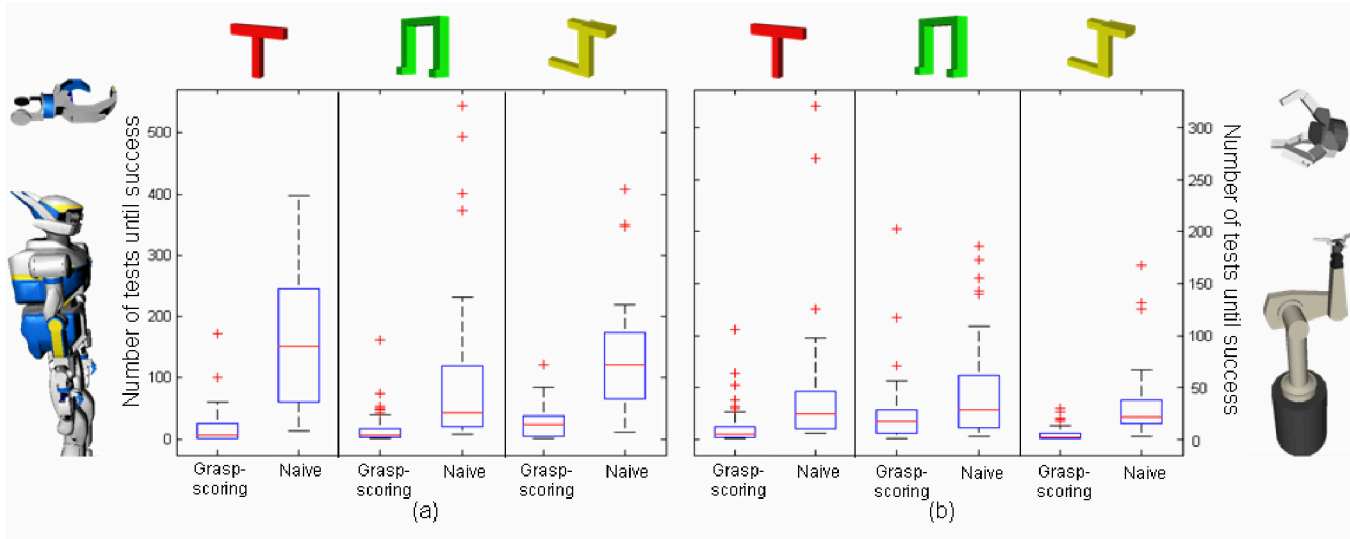
Figure 14.4: Box plot of the statistics for the benchmark experiment on the three objects for the HRP2 and Puma robots. Objects 1, 2, and 3 shown at the top (left to right) were placed in 50 random scenes. The vertical axis is the number of grasps tried before a successful one was found. The red line in each box plot represents the number of tests necessary to find a successful grasp averaged over the 50 scenes. Lower is better. (a) Statistics when using the HRP2. (b) Statistics when using the Puma+Barrett hand robot.
