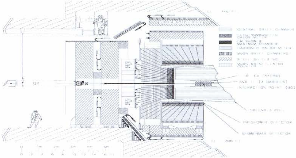
Figure 7: The CDF Run II Detector
