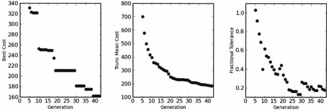
Figure 24: Convergence history for the 'b-jet' particle content tuning.
