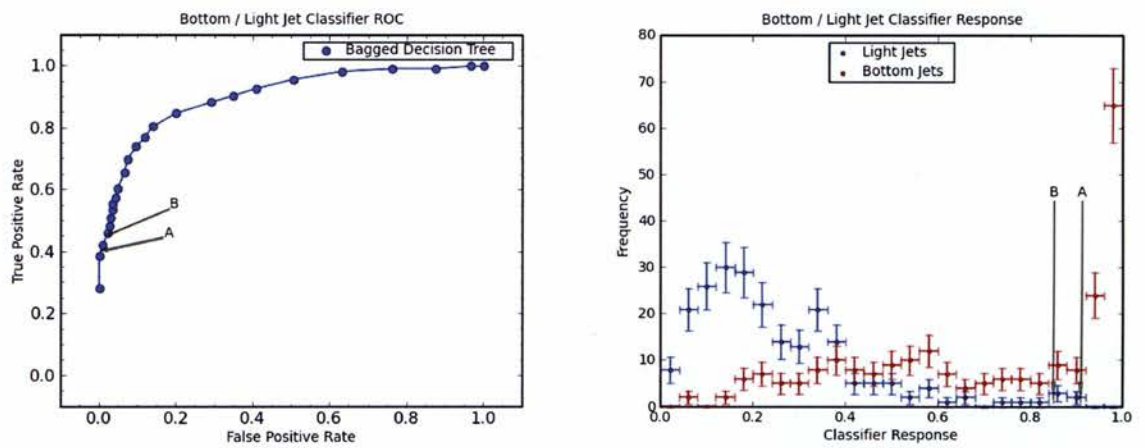
Figure 40: The performance of the bottom vs light flavor jet classifier on validation MC.
