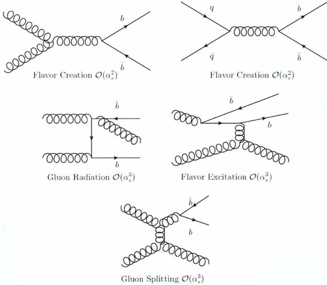
Figure 1: Example diagrams for Standard Model b\bar{b} production at the TeVatron
