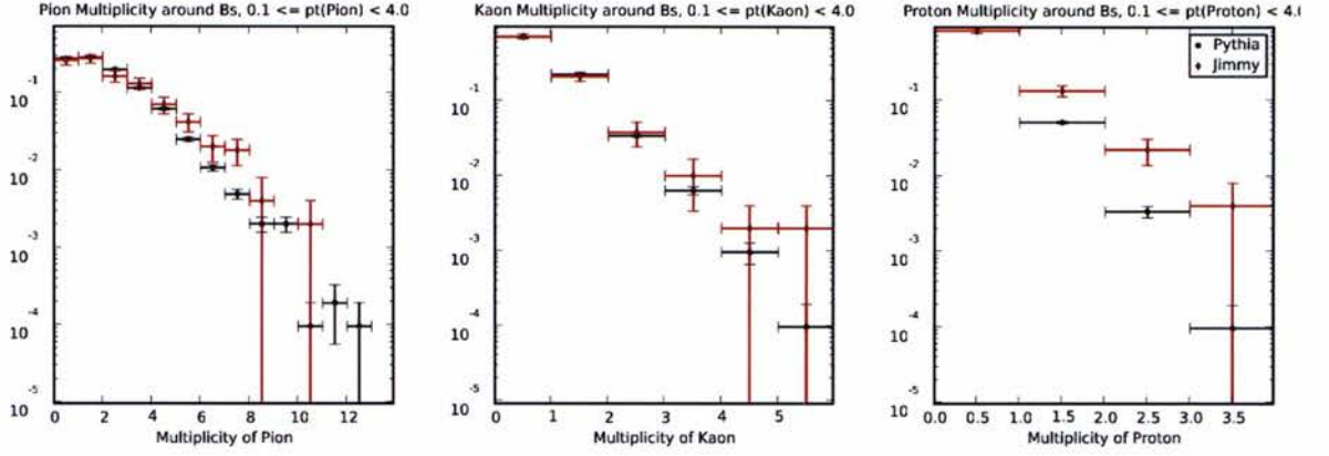
Figure 26: BJet Tune results: track multiplicity around B_s mesons.
