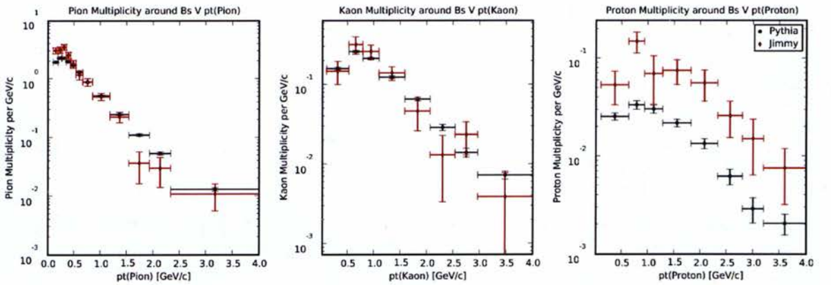
Figure 28: BJet Tune results: track multiplicity around B_s mesons vs p_T(\text{track})
