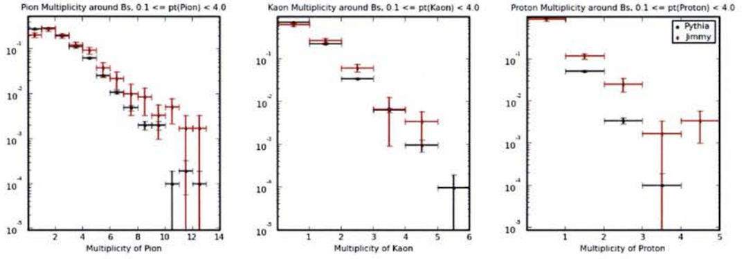
Figure 19: HERWIG Defaults: track multiplicity around B_s mesons.
