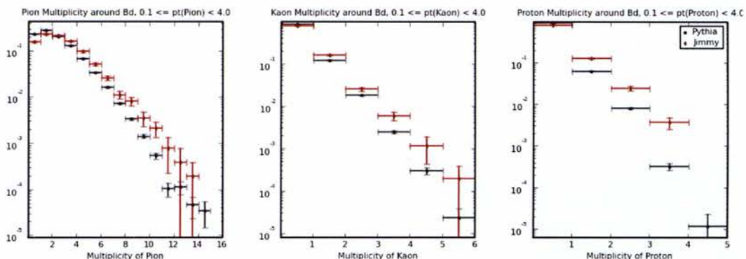
Figure 18: HERWIG Defaults: track multiplicity around B_d mesons.
