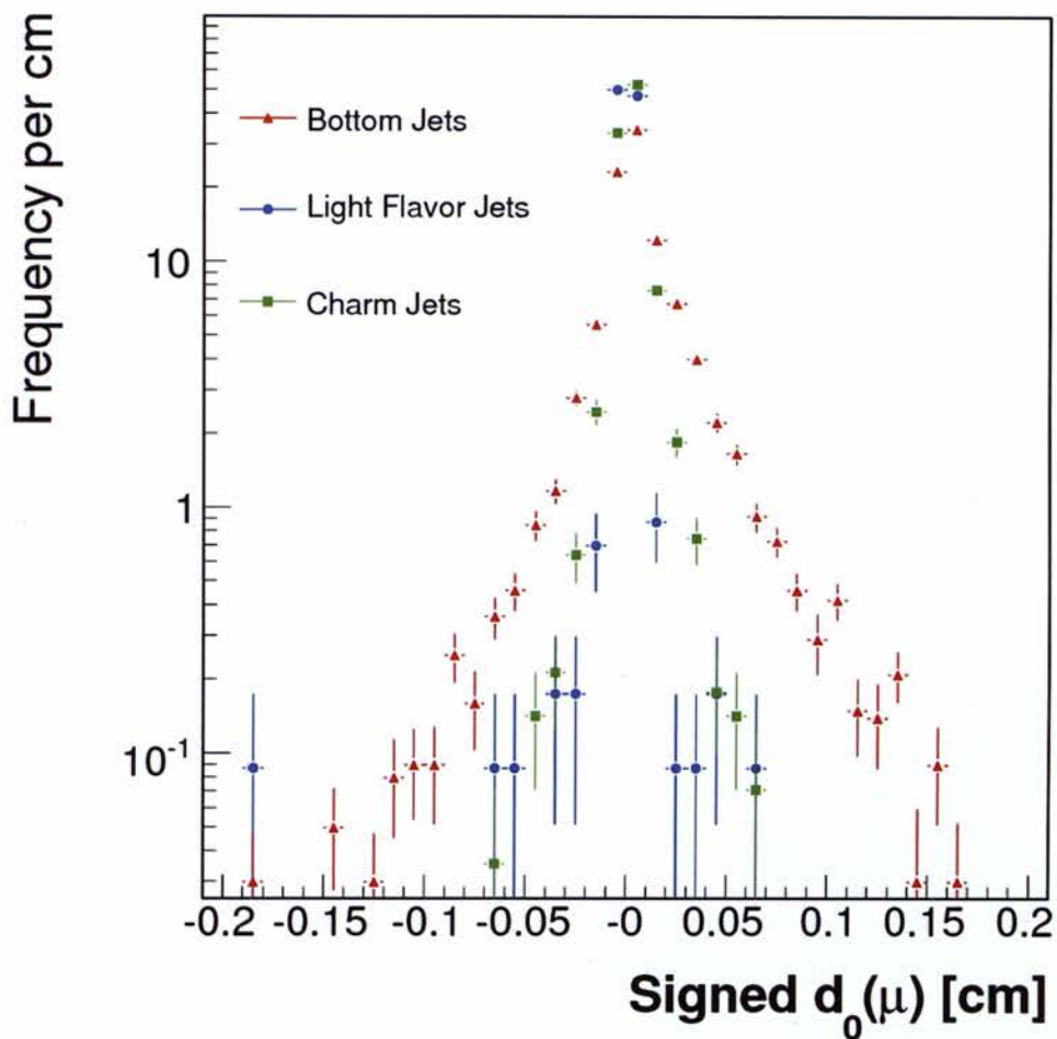
Figure 35: Muon jet-signed d_0 from bottom hadron decay (red triangles), charm hadron decay (green squares), and light flavor sources (blue circles; includes decay-in-flight and punch through muons). Histograms are normalized to unit area.
