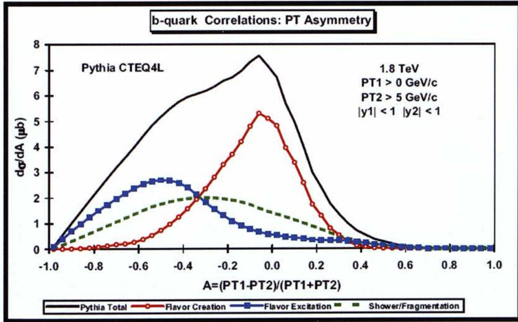
Figure 3: Bottom quark pair transverse momentum asymmetry \mathcal{A}_{pT}(b, \bar{b}) , from Ref. [5]
