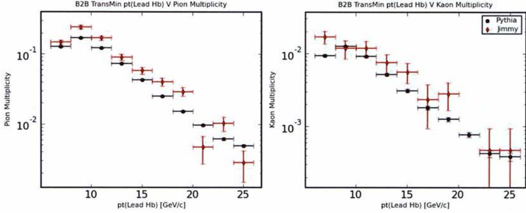
Figure 13: UE Defaults: charged pion (left) and charged kaon (right) multiplicity vs p_T(\text{Lead } H_b) .
