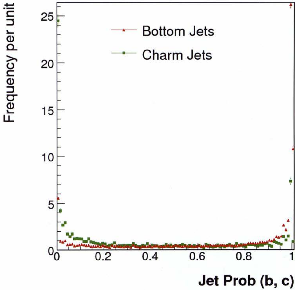
Figure 43: Generalized Jet Probability for bottom jets (red triangles) and charm jets (green squares) for bottom vs light jet operating point A on validation MC. Histograms are normalized to unit area.
