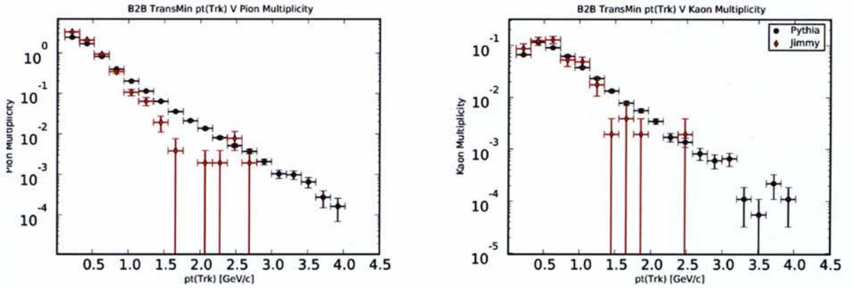
Figure 30: UE tune results (after BJetTune): charged pion multiplicity vs p_T(\pi^\pm) (left) and charged kaon multiplicity vs p_T(K^\pm) (right).
