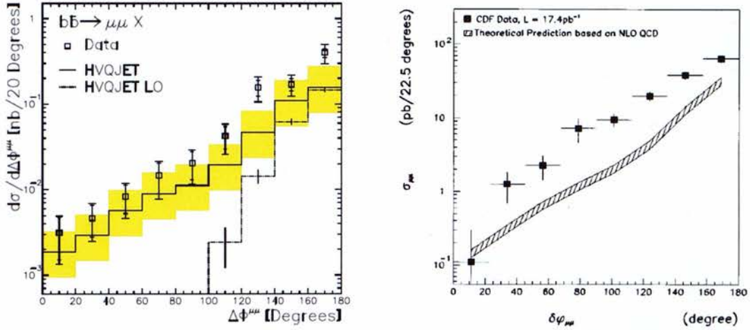
Figure 5: Dimuon correlations at the TeVatron; the DØ [38] result is on the left, and the CDF [39] is on the right.
