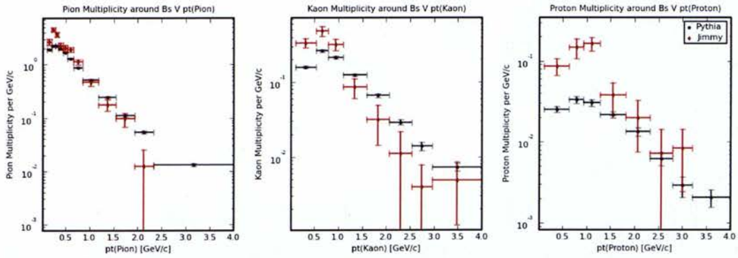
Figure 21: HERWIG Defaults: track multiplicity around B_s mesons vs p_T (track)
