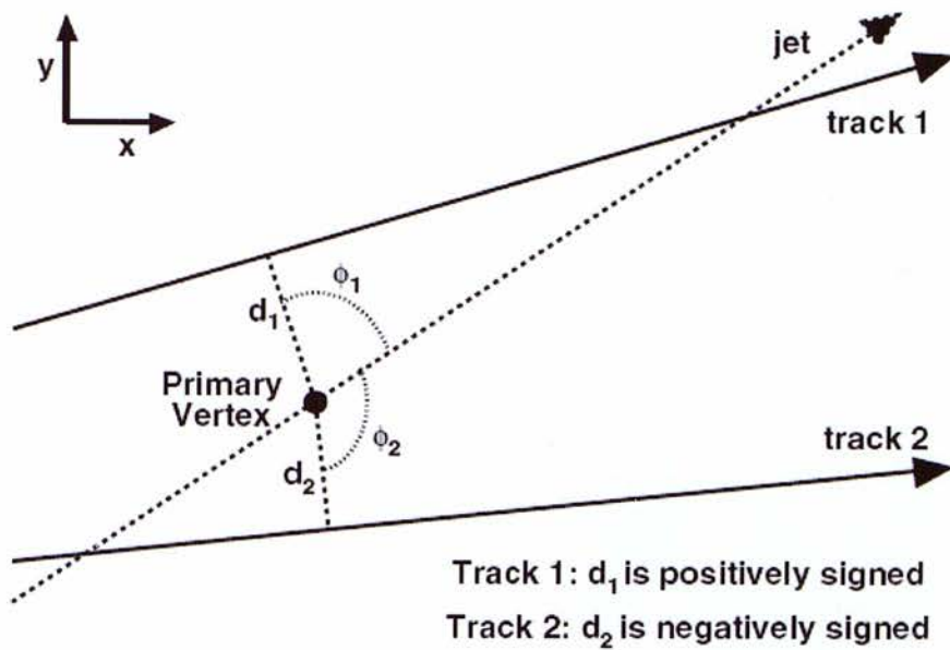
Figure 34: Definition of jet-signed d_0 , taken from Ref. [49].
