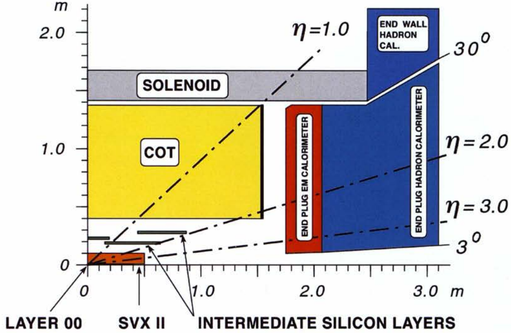
Figure 9: An r - z view of the CDF Run II tracking detectors.
