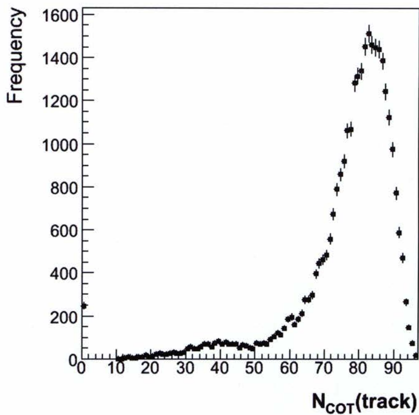
Figure 32: Distribution of the number of COT hits for tracks within \mu -jets from CDF data.
