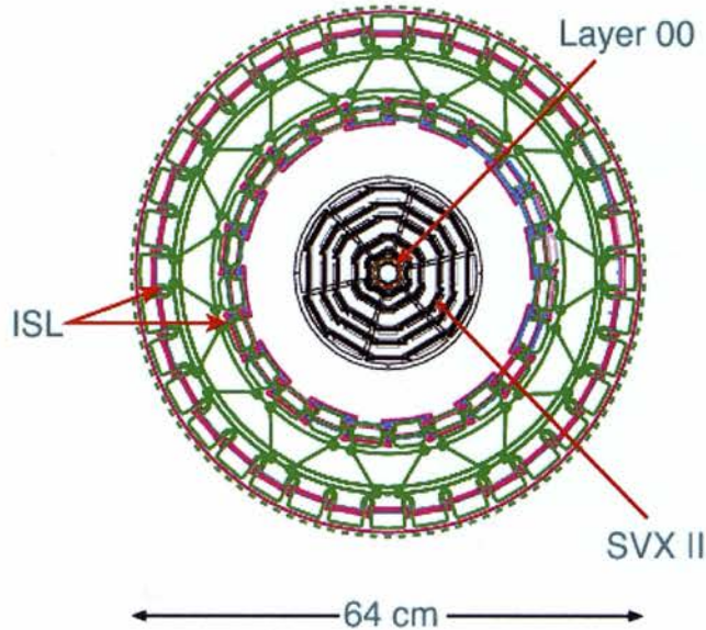
Figure 8: An end view of the CDF Run II silicon detectors.
