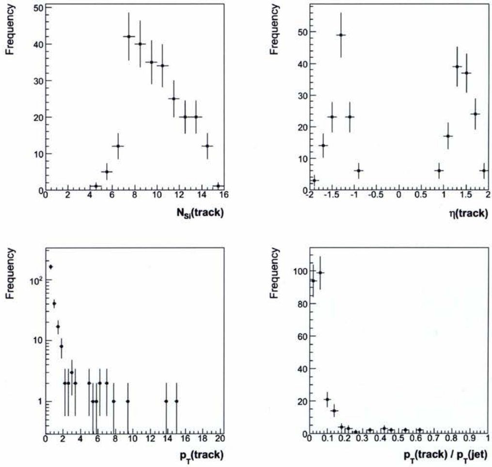
Figure 33: Silicon stand-alone track characteristics in CDF data.
