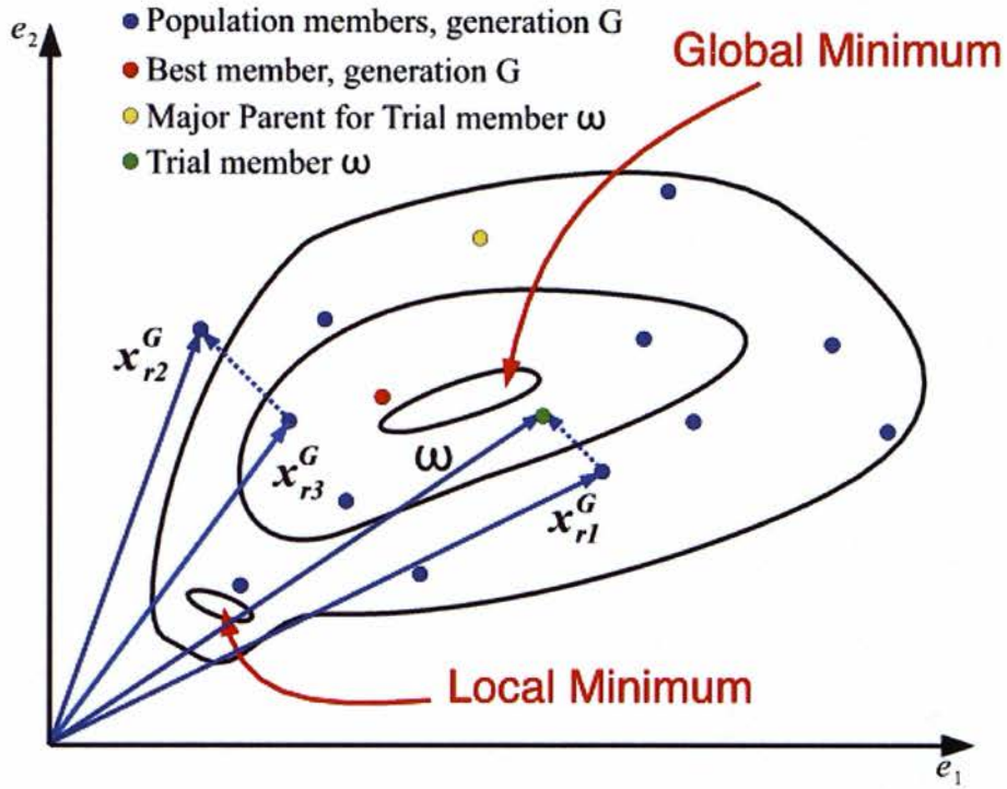
Figure 11: An example of the mutant \omega construction using DE/rand for a two-dimensional objective function.
