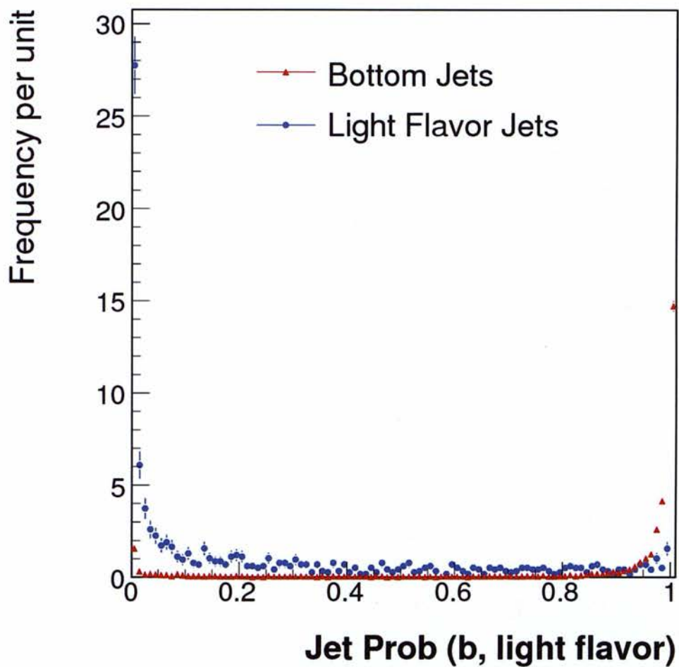
Figure 38: Generalized Jet Probability for bottom jets (red triangles) and light flavor jets (blue circles). Histograms are normalized to unit area.
