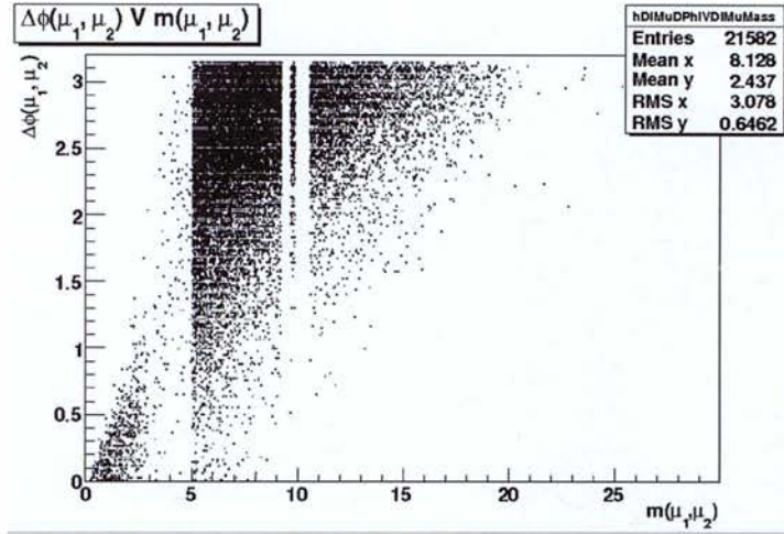
Figure 31: \Delta\phi(\mu_1, \mu_2) vs m(\mu_1, \mu_2) for MC@NLO semi-muonic b\bar{b} events which pass the trigger and good muon selection of Section 8.3 (no jet criteria are applied). The majority of events with \Delta\phi(\mu_1, \mu_2) < 0.7 fail the mass requirement imposed by the trigger ( m(\mu_1, \mu_2) > 5 GeV/ c^2 ).
