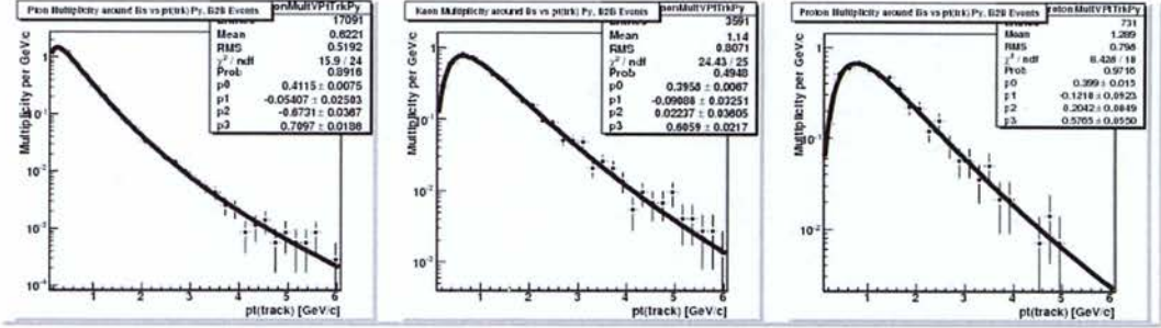
Figure 23: Log-normal fits to the PYTHIA TuneA multiplicity vs p_T(\text{particle}) for pions (left), kaons (middle), and protons(right) around B_s mesons.
