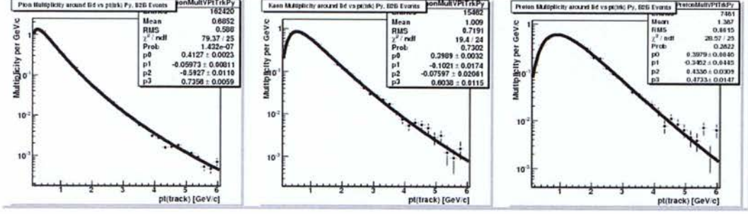
Figure 22: Log-normal fits to the PYTHIA TuneA multiplicity vs p_T(\text{particle}) for pions (left), kaons (middle), and protons(right) around light bottom mesons ( B_d and B_u ).
