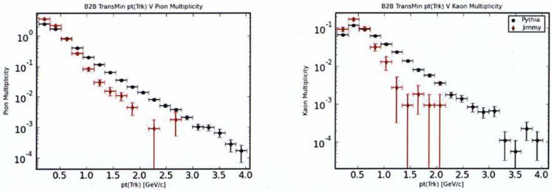
Figure 17: UE tune results: charged pion multiplicity vs p_T(\pi^\pm) (left) and charged kaon multiplicity vs p_T(K^\pm) (right).
