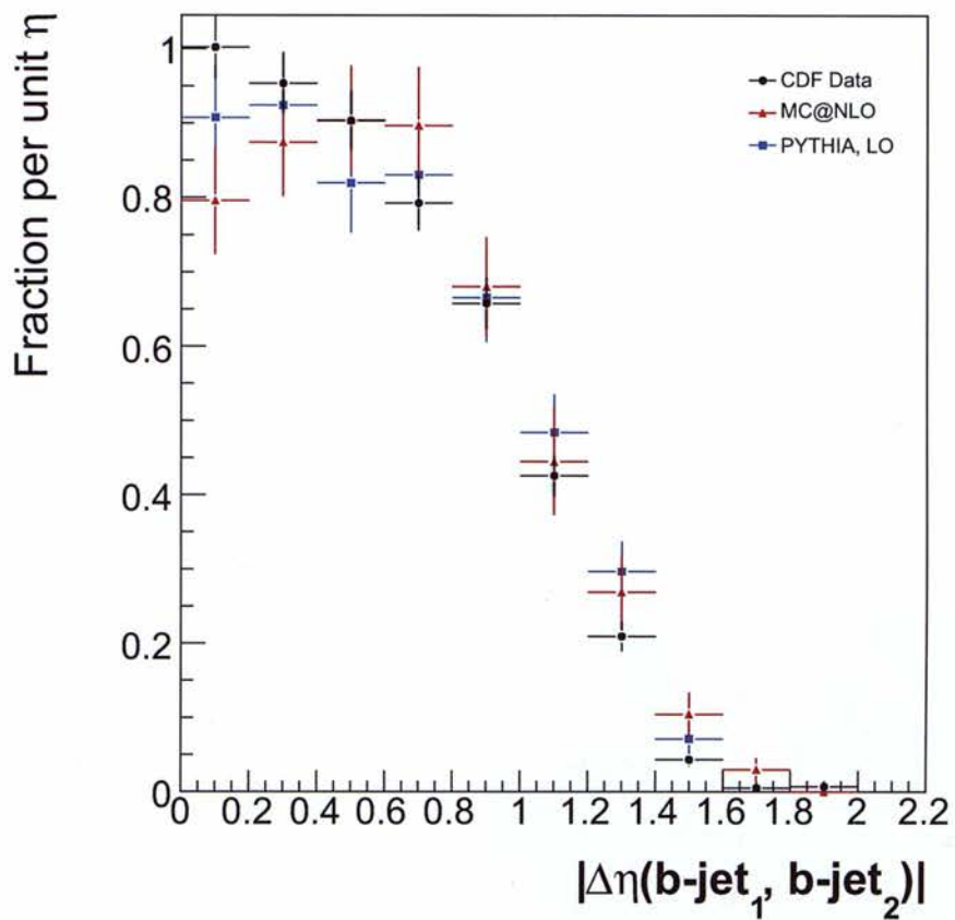
Figure 54: |\Delta\eta| between the two b -jets for data (black points), MC@NLO (red triangles), and LO PYTHIA (blue squares).
