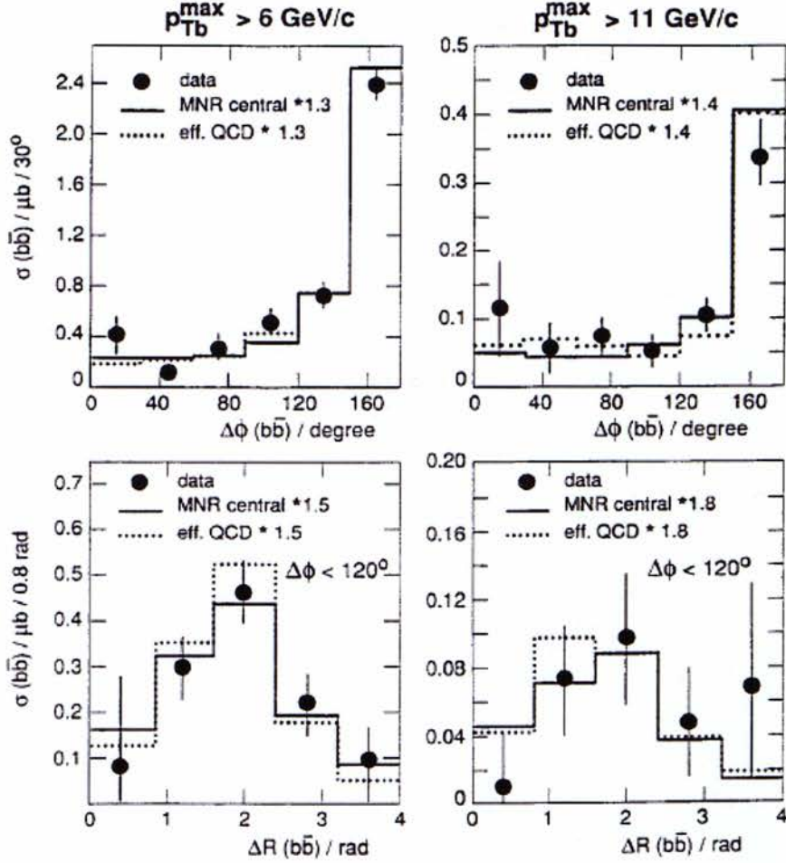
Figure 4: Measured b\bar{b} angular correlations, compared with MNR NLO theory and a parton shower MC (labeled 'eff. QCD' in the legends), from Ref. [33]. The plots on the left were made with a minimum p_{Tb} of 6 GeV/c for the highest p_T quark in each event, while the minimum p_{Tb} threshold for the plots on the right was set at 11 GeV/c. The top row shows the \Delta\phi(b, \bar{b}) , while the bottom row shows \Delta R(b, \bar{b}) for \Delta\phi(b, \bar{b}) < 120^\circ . This latter requirement removes all of the flavor creation component.
