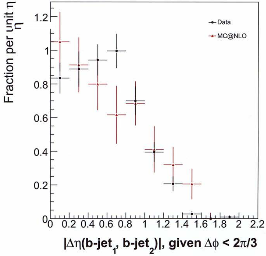
Figure 53: |\Delta\eta| between the two b -jets, given \Delta\phi < 2\pi/3 for data (black points) and MC@NLO (red triangles).
