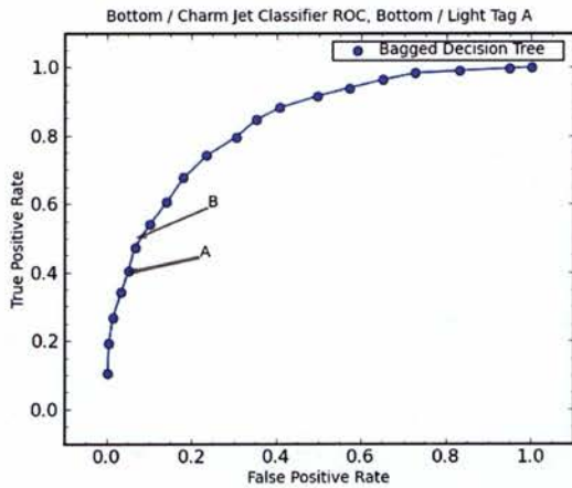
Figure 46: The performance of the bottom vs charm jet classifier for bottom vs light jet operating point A on validation MC.
