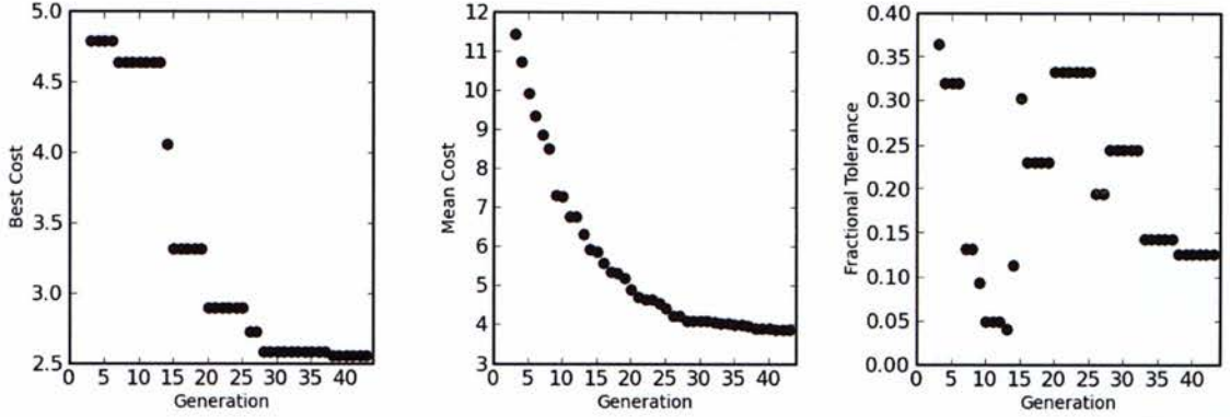
Figure 15: UE tune convergence history
