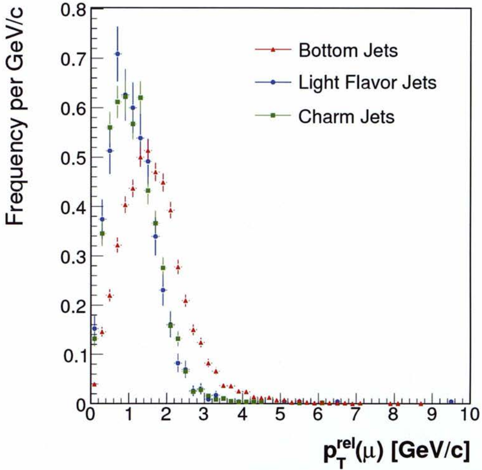
Figure 36: The relative transverse momentum p_T^{\text{rel}} for muons from bottom hadrons (red triangles), muons from charm hadrons (green squares), and muons from light flavor sources (blue circles; includes decay-in-flight and punch through muons). Histograms are normalized to unit area.
