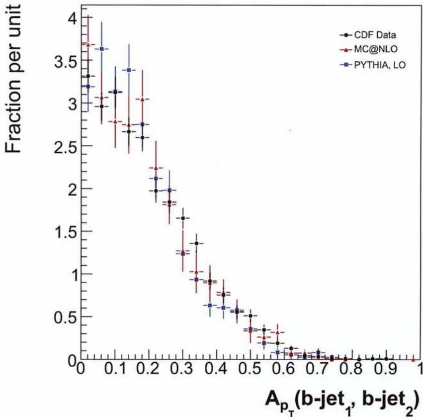
Figure 52: \mathcal{A}_{p_T} for the two b -jets for data (black points), MC@NLO (red triangles), and LO PYTHIA (blue squares).
