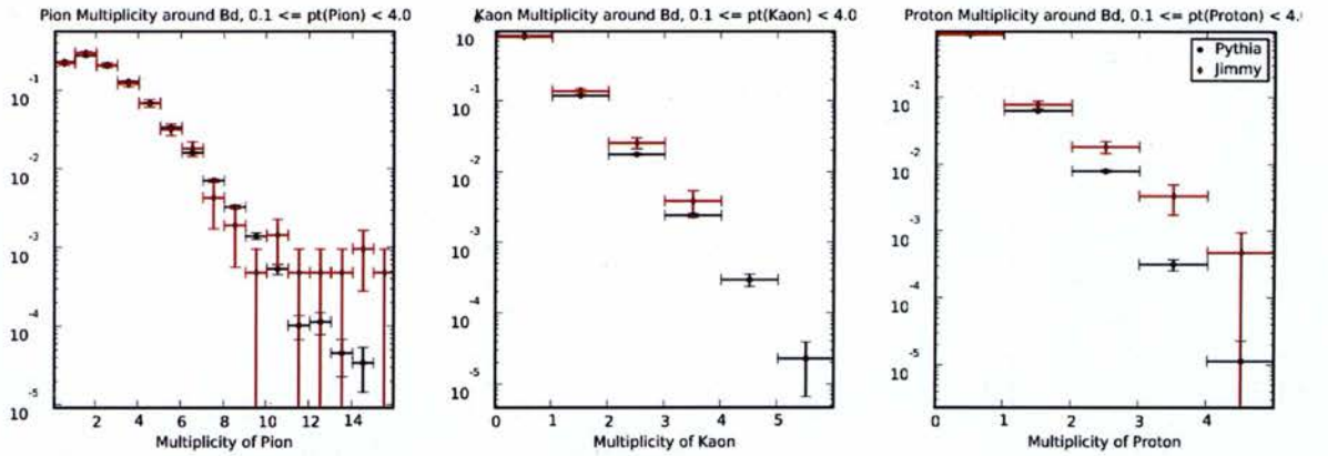
Figure 25: BJet Tune results: track multiplicity around B_d mesons.
