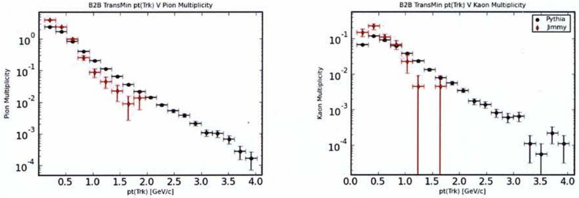
Figure 14: UE Defaults: charged pion multiplicity vs p_T(\pi^\pm) (left) and charged kaon multiplicity vs p_T(K^\pm) (right).
