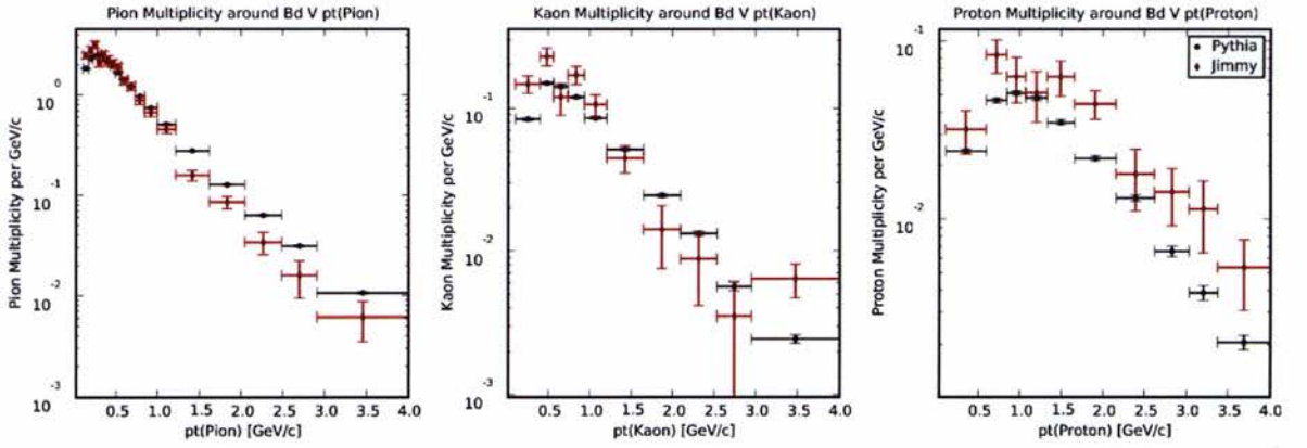
Figure 27: BJet Tune results: track multiplicity around B_d mesons vs p_T(\text{track})
