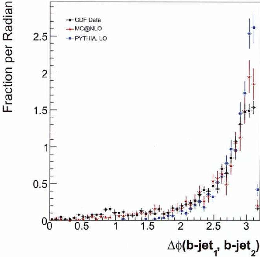
Figure 50: \Delta\phi between the two b -jets for data (black points), MC@NLO (red triangles), and LO PYTHIA (blue squares).
