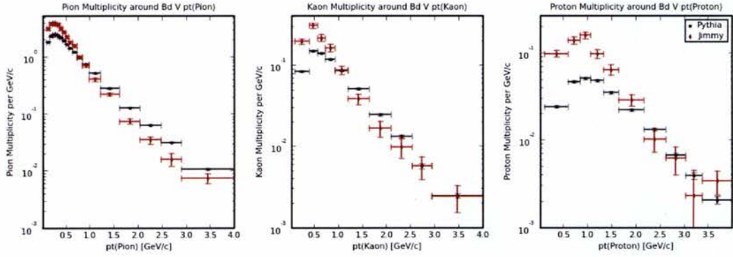
Figure 20: HERWIG Defaults: track multiplicity around B_d mesons vs p_T (track)
