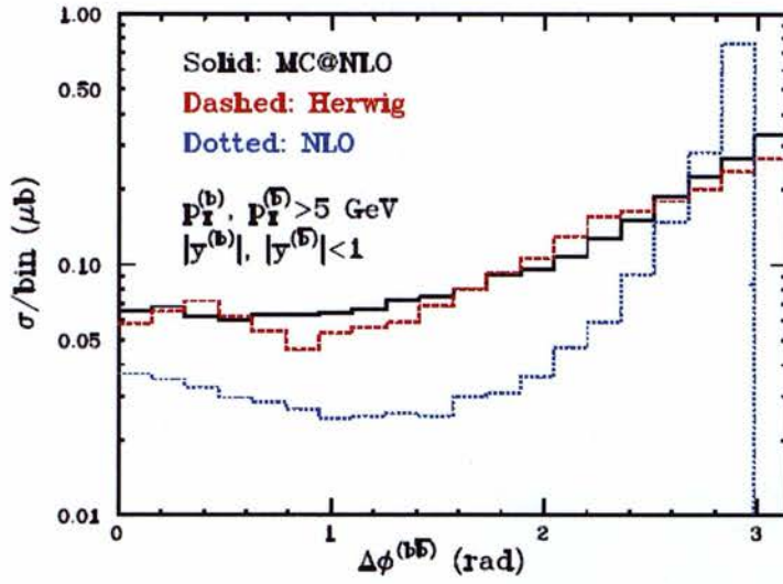
Figure 51: Azimuthal angular difference between bottom quarks with the requirements p_T(b) > 5 \text{ GeV}/c and |y(b)| < 1 for MC@NLO (solid), HERWIG (dashed), and partonic NLO theory (dotted).
