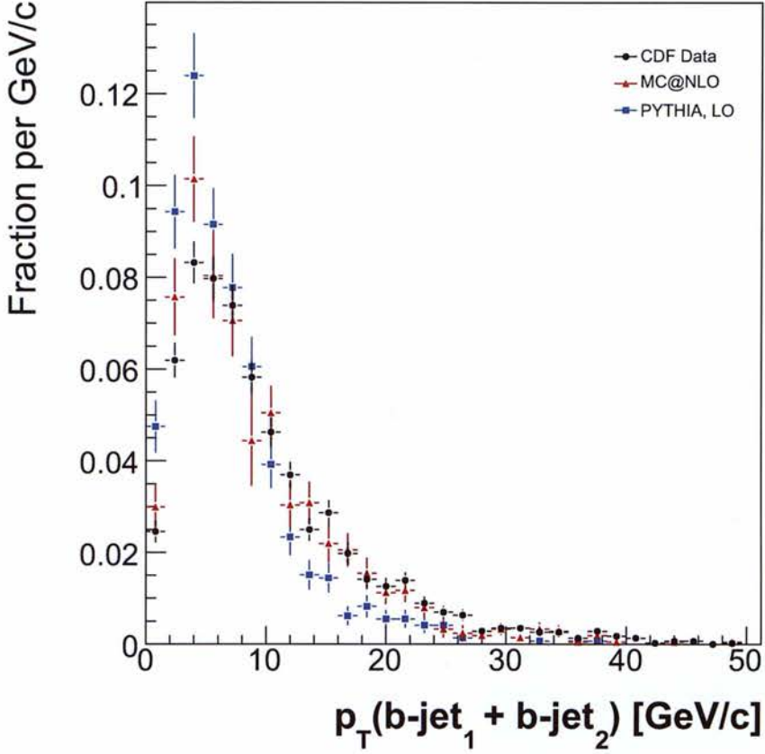
Figure 48: p_T of the b -jet system for CDF data (black points), MC@NLO (red triangles), and LO PYTHIA (blue squares).
