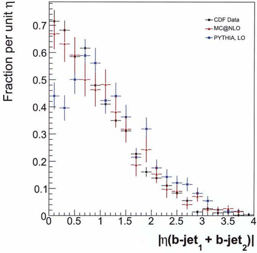
Figure 49: |\eta| of the b -jet system for CDF data (black points), MC@NLO (red triangles), and LO PYTHIA (blue squares).
