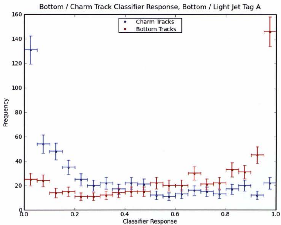
Figure 41: The performance of the bottom vs charm track classifier for bottom vs light jet operating point A on validation MC.
