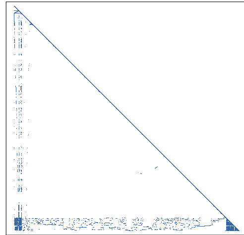
(b) Groupings: (pose) (landmark), 4156978 nonzero entries
