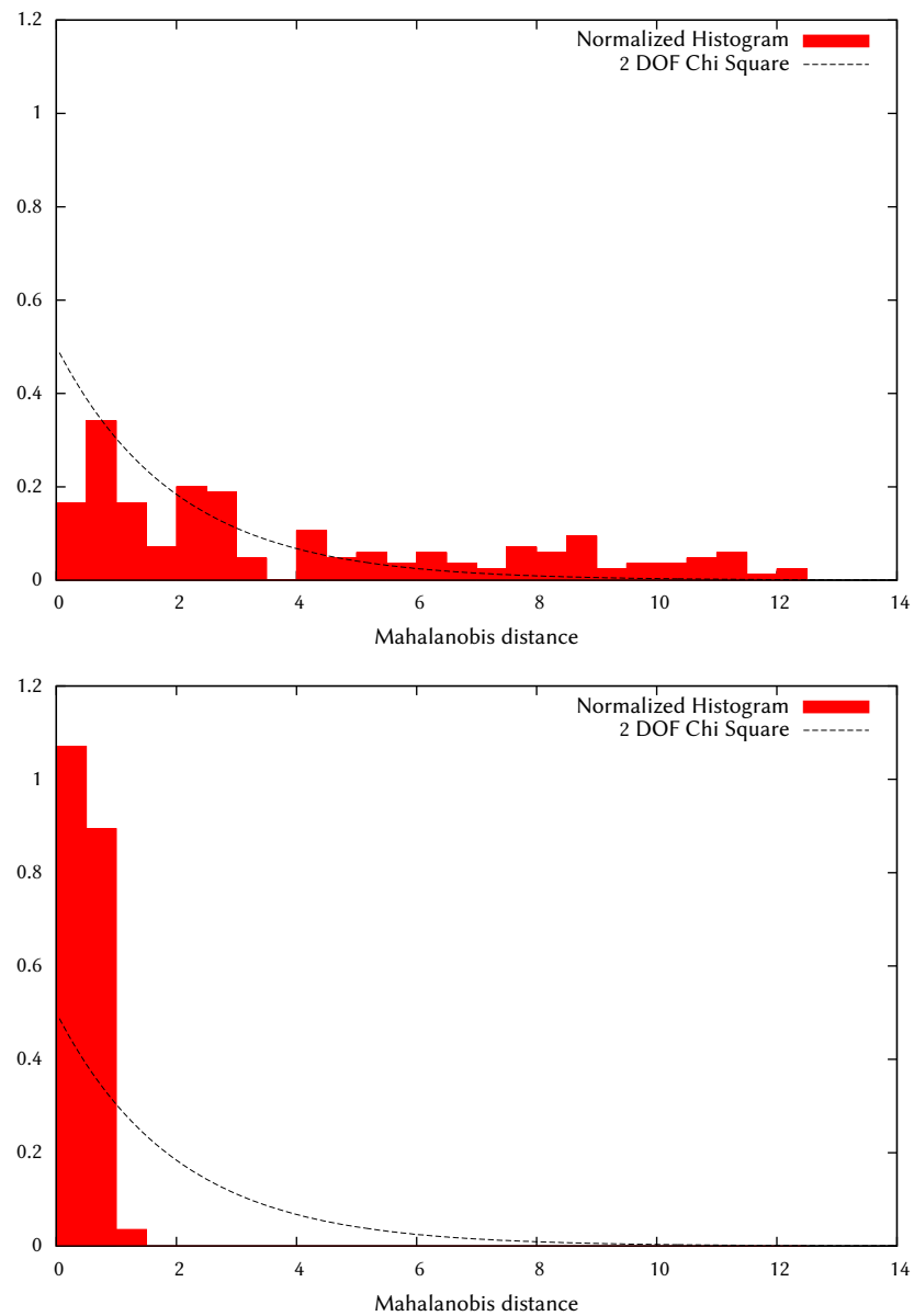
Figure 6.6.6: Mahalanobis distances between estimates of the location of the same landmark using multiple datasets. Ideally, the distances should be drawn from a chi square distribution with 2 degrees of freedom. The top histogram is the divergent result when the naive independence assumption is used. The bottom histogram shows the conservative, but consistent results when using explicit bias estimation.
