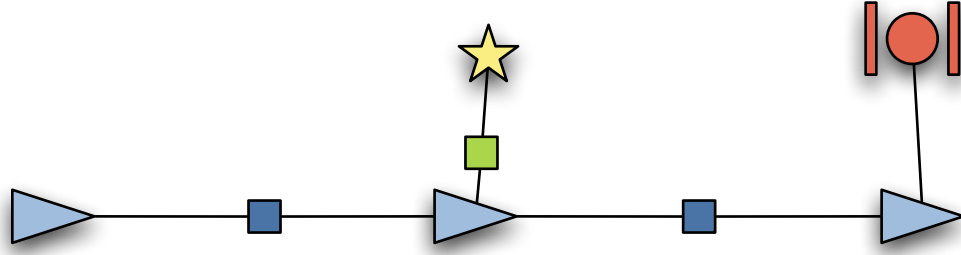
Figure 5.3.1: An example trajectory chain without a prior for the first pose. The robot begins operating, but has no information about its global location. After moving, it observes a landmark, and after moving again it receives GPS information.
