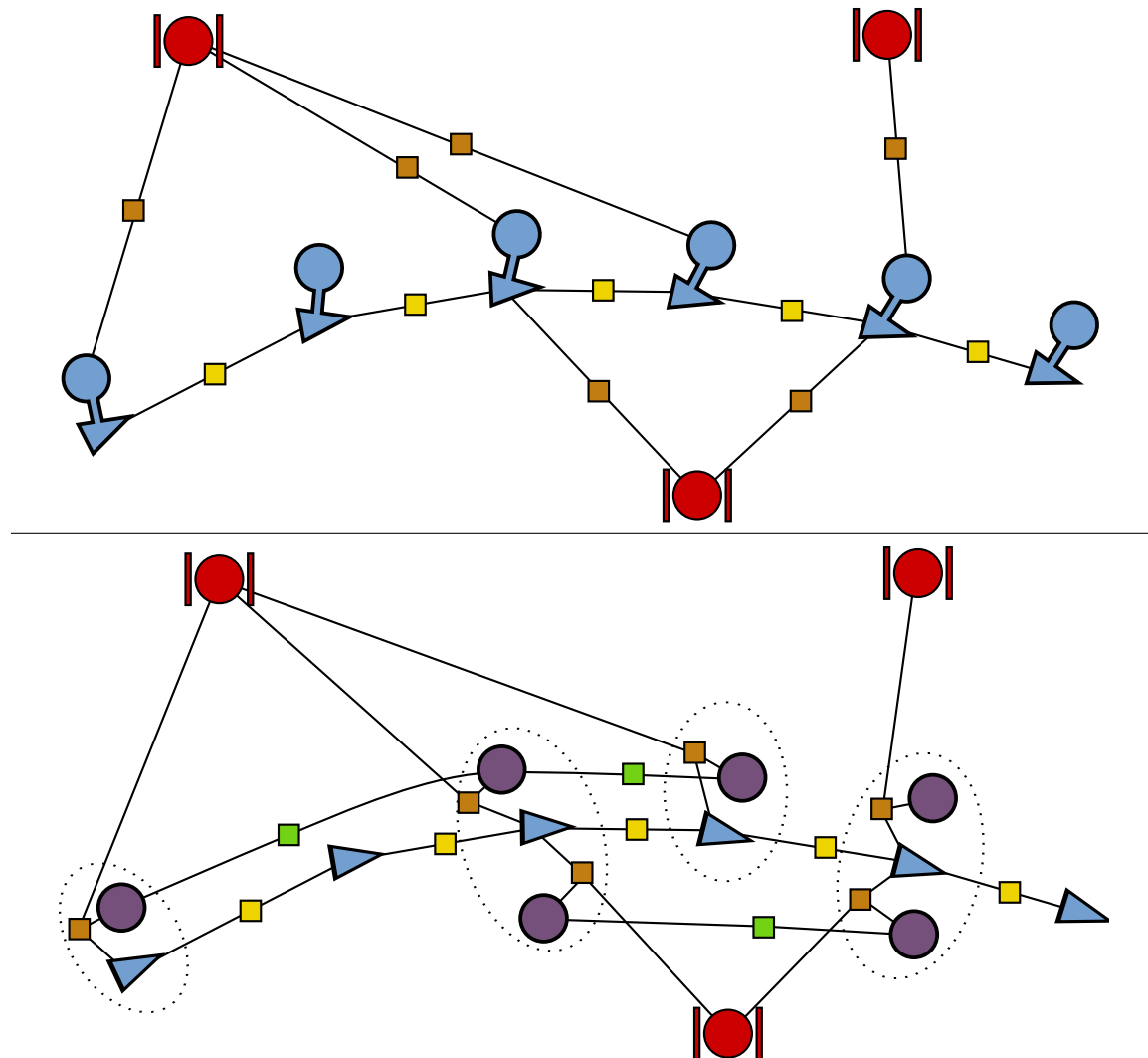
Figure 5.3.2: Factor graphs of two bias augmentation strategies. Constraints from process models or measurements are represented by small squares. The top diagram shows the least invasive way to augment the system mathematically: augmenting the robot state with bias information and propagating this through the existing process model. This has an appealing simplicity but hides significant inefficiency; since the entire set of biases is estimated at every pose step. The lower figure illustrates separating out the bias process model to avoid adding unnecessary terms to the system; biases are estimated only when we take a reading from the associated satellite. The dotted lines group terms which are coincident in time. (Note: landmarks have been omitted for clarity, and satellite representations are included to clarify groupings; they do not represent variables being estimated.)
