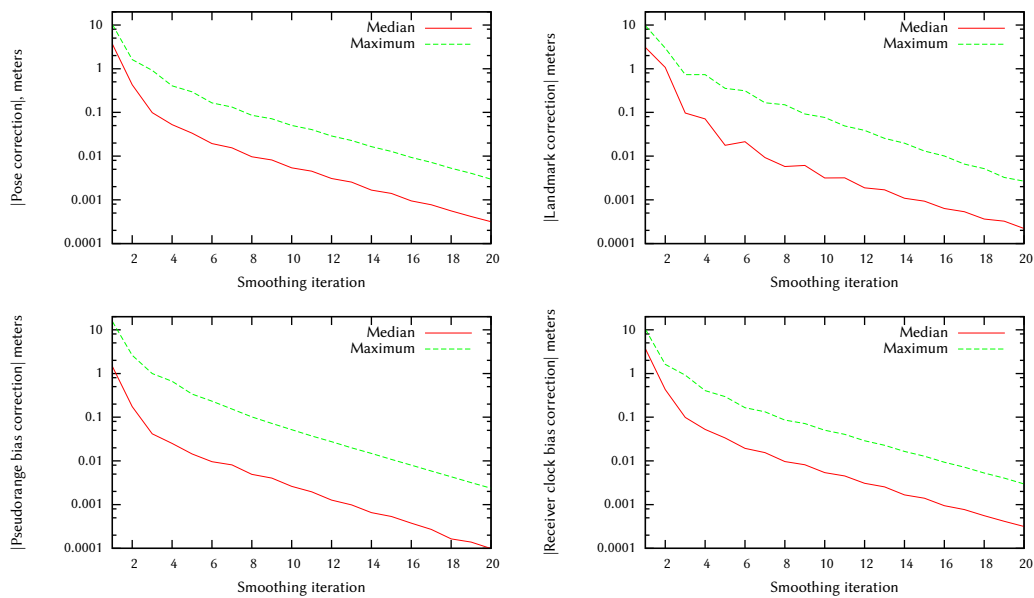
Figure 6.7.4: Convergence rates of the various types of parameters being estimated in the Pittsburgh dataset without differential corrections. Scale is logarithmic.
