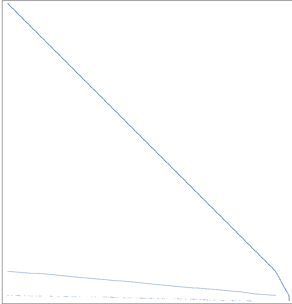
Figure 6.7.5: The A matrix of the full mapping run. The top rows of the matrix are the pose updates. These are followed by the GPS observations and then the landmark observations. Columns are poses, then clock offsets and satellite biases, then landmark positions. The matrix is 245498 \times 232094 , and contains 1890688 nonzero entries.
