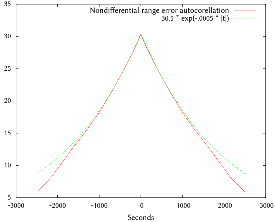
Figure 3.5.2: Autocorrelation of raw satellite pseudorange error
