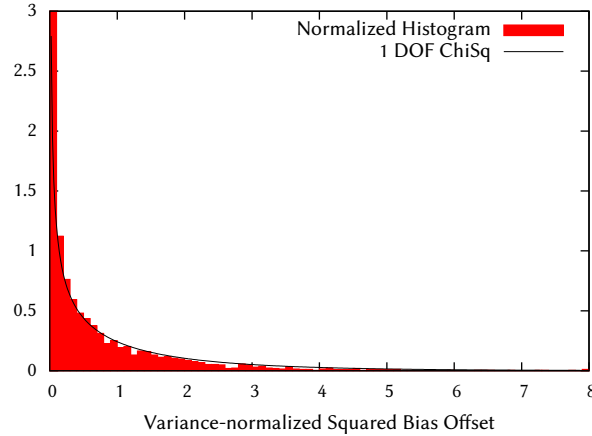
Figure 6.8.3: Normalized histogram of variance-normalized satellite offsets.
