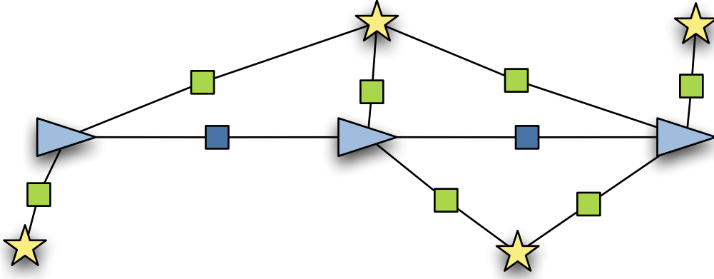
Figure 5.2.1: Factor graph for the scenario in 5.2.22. The system involves 3 poses (triangles), 4 landmarks (stars), 7 landmark observations (green boxes) and 2 motion updates (blue boxes).
