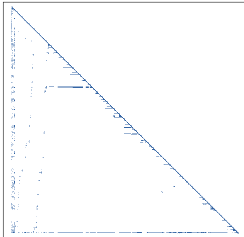
(c) Groupings: (pose) (landmark) (gps), 5656914 nonzero entries
