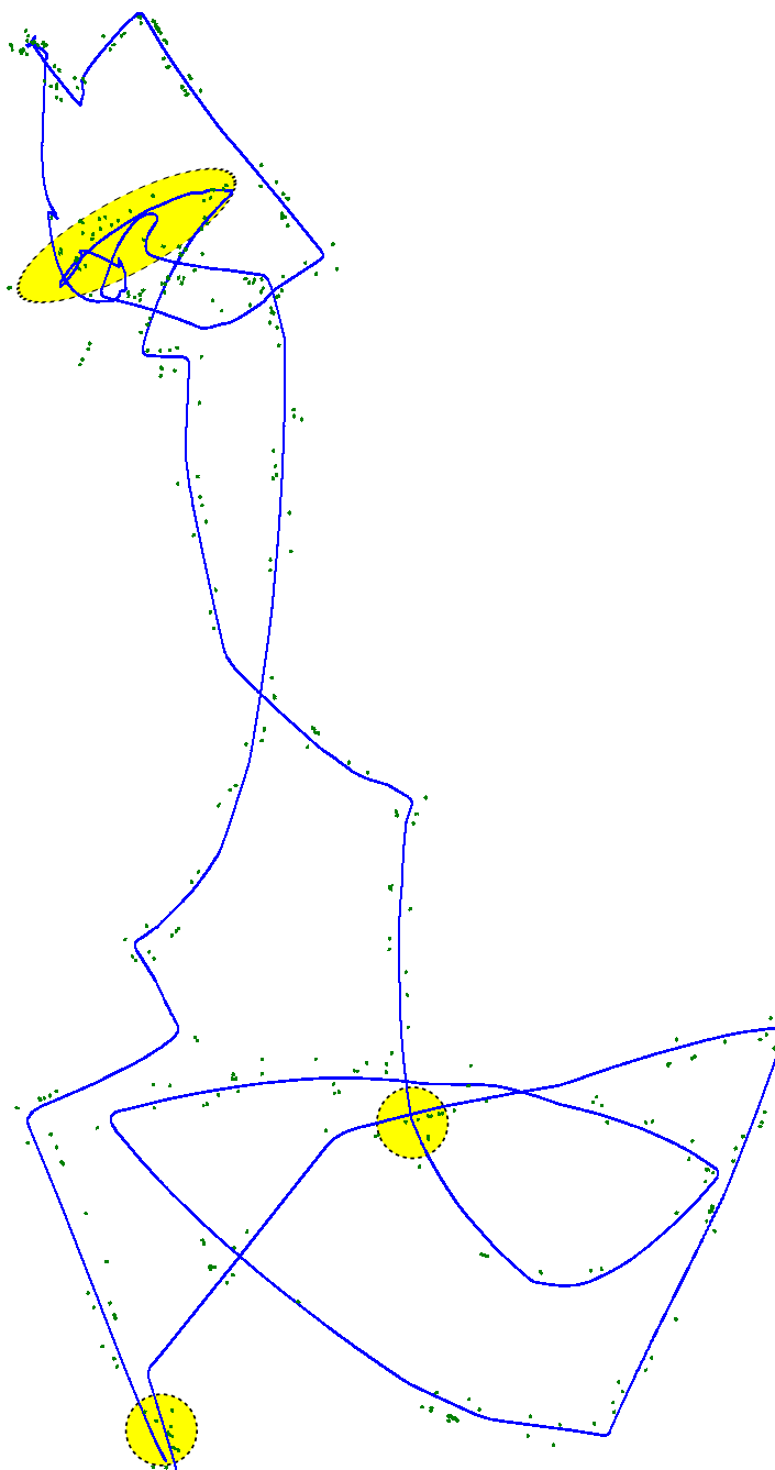
Figure 6.6.3: Results of smoothing using odometry, oracular data associations and Levenberg Marquardt descent. Several loop closures have been highlighted with yellow circles. Even relatively small examples do not converge to a correct map.
