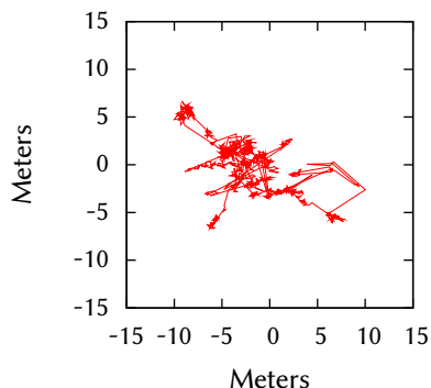
Figure 3.3.1: East-North-Up coordinate frame fixes every 30 seconds over an 8-hour window from using a base station with a fixed antenna. Modeling the outputs of this system is a decidedly nontrivial task.
