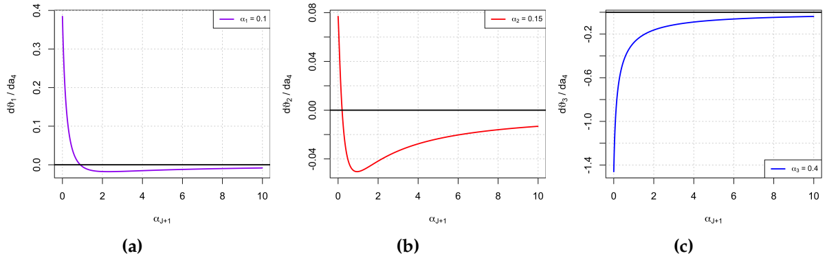
Figure 3.3.: From left to right we show \frac{d\boldsymbol{\vartheta}_{iyt}^*}{da_{i4t}} where y \in (1, 2, 3) as a function of the marginal propensity to save \alpha_{i,J+1} . In panel (a) the value of \alpha_{ij} associated with good y = 1 is 0.1, in panel (b) it is 0.15, and in panel (c) it is 0.4. Notice that depending on \alpha_{ij} and \alpha_{i,J+1} optimal budget updates respond differently to over or under spending in the non-updated, sparse category \Gamma_{i4t} = 0 .
