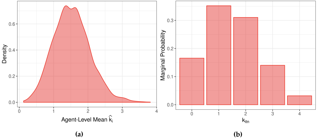
Figure 3.6.: In panel (a) we present the posterior density of \hat{k}_i = \frac{1}{NT_i} \sum_n \sum_t \sum_j \Gamma_{ijtn} , i.e. the number of budget changes each period averaged over time and across MCMC draws for each agent, using a smoothed Gaussian kernel with the Silverman rule-of-thumb for choosing the bandwidth (Silverman 1986). In panel (b) we show the marginal posterior probability mass function for the atomic draws of k_{itn} .
