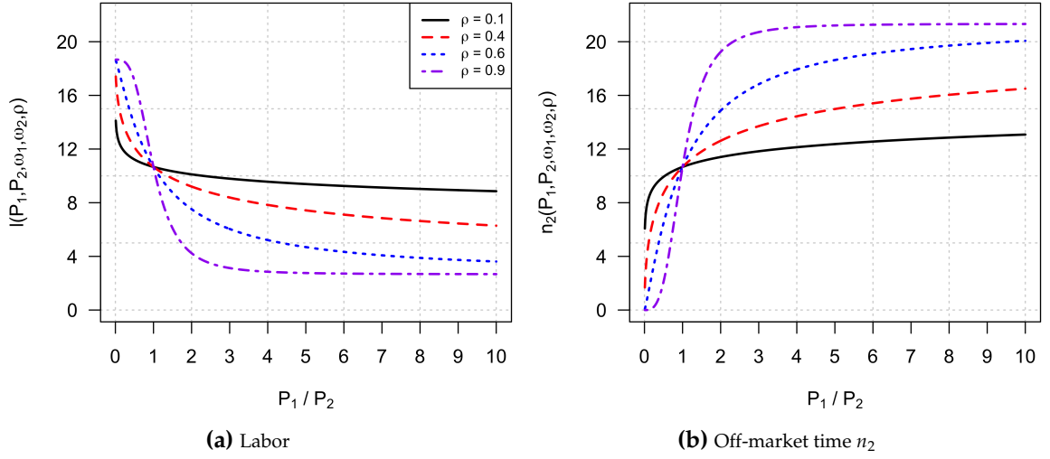
Figure 1.3.: ( 0 < \rho < 1 and \omega_1 > \omega_2 ) — Here, we set \omega_1 = 0.8 and \omega_2 = 0.2 , so that process i = 2 is more time intensive. Notice that increasing P_1 relative to numeraire P_2 causes l to fall. As \rho \rightarrow 1 , home production outputs become more substitutable, and the strength of this substitutability dominates complementarities between market purchases and time use.
