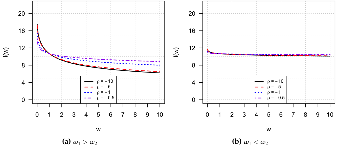
Figure 1.8.: ( \rho < 0 ) — Here we present household labor supply variation in w for the case when home production outputs are complements. In panel (a) \omega_1 = 0.8 and \omega_2 = 0.2 , so that process i = 2 is more time intensive. In panel (b) \omega_1 = 0.4 and \omega_2 = 0.6 , so that process i = 1 is more time intensive but to a lesser magnitude than as in panel (a). Labor supply appears to be non-increasing in w for all values of \rho < 0 .
