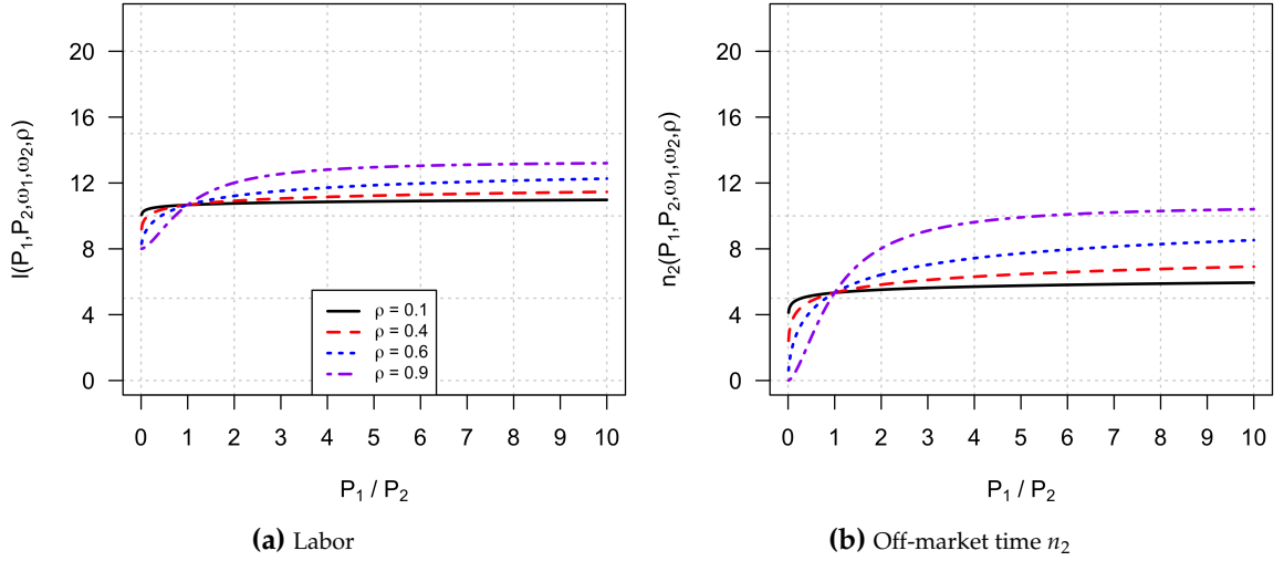
Figure 1.4.: ( 0 < \rho < 1 and \omega_1 < \omega_2 ) — This time we set \omega_1 = 0.4 and \omega_2 = 0.6 , so that process i = 1 is more time intensive. As \rho \rightarrow 1 , approaching linear preferences for final consumption, n_2 begins to increase in P_1/P_2 to the point where for \rho = 0.9 , the n_2 policy function appears monotonic in P_1/P_2 . As \rho \rightarrow 0 consumers compensate for declines in q_1 by spending more time on process i = 1 .
