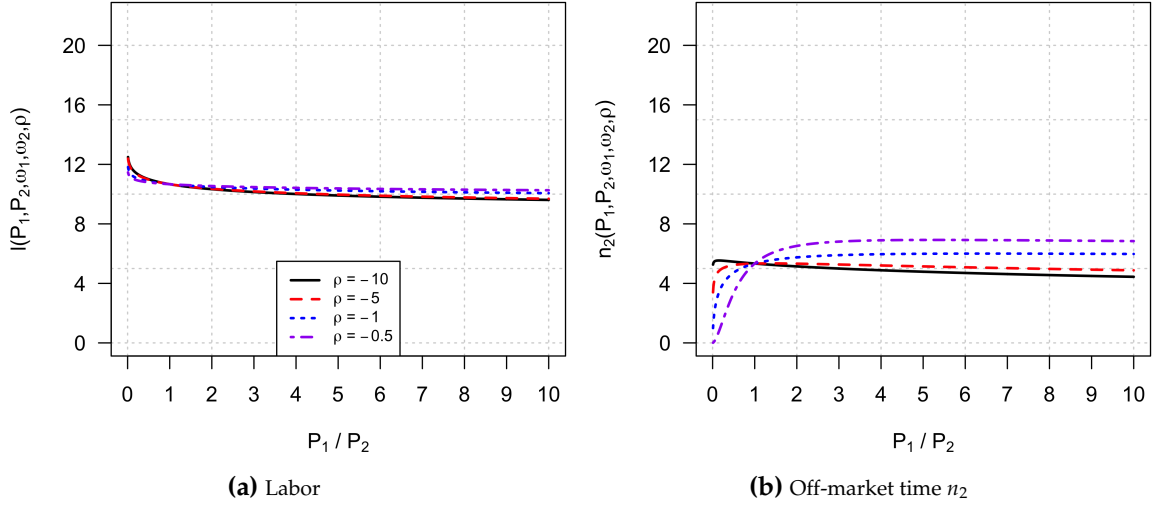
Figure 1.6.: ( \rho < 0 and \omega_1 < \omega_2 ) — As in Figure 1.4 we set \omega_1 = 0.4 and \omega_2 = 0.6 , so that now process i = 1 is more time intensive. Labor supply is flat in prices again and n_2 exhibits very small variation, similar to when \rho \in (0, 1) . Notice that, though when \rho \in (0, 1) there appears to be a limiting condition in which increases in P_1 lead to changes in the behavior of n_2 , this does not occur when \rho < 0 .
