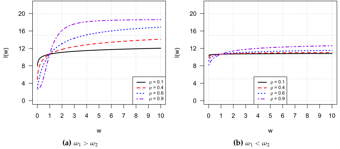
Figure 1.7.: ( 0 < \rho < 1 ) — Here we present household labor supply variation in w for the case when home production outputs are substitutes. In panel (a) \omega_1 = 0.8 and \omega_2 = 0.2 , so that process i = 2 is more time intensive. In panel (b) \omega_1 = 0.4 and \omega_2 = 0.6 , so that process i = 1 is more time intensive but to a lesser magnitude than as in panel (a). Labor supply appears to be non-decreasing in w for all values of \rho \in (0, 1) .
