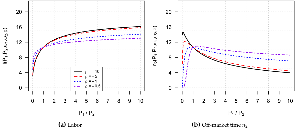
Figure 1.5.: ( \rho < 0 and \omega_1 > \omega_2 ) — Now final activities are complements. As in Figure 1.3 we set \omega_1 = 0.8 and \omega_2 = 0.2 , so that process i = 2 is more time intensive. Labor varies in P_1/P_2 in the opposite way than when \rho \in (0, 1) . Further, n_2 declines in P_1/P_2 faster than l rises, so that the remaining time moves to process i = 1 , the task for which the market input experienced a price increase.
